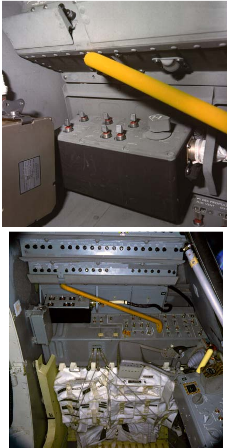
Figure 8 - Top photo shows the DSEA in its mounted position inside LM-11 (Apollo 16's LM "Orion") during final closeout. The bottom photo shows the DSEA's relative position behind the commander's station onboard a LM trainer. NASA Photo No. S72-35124 and No. S70-30949.
