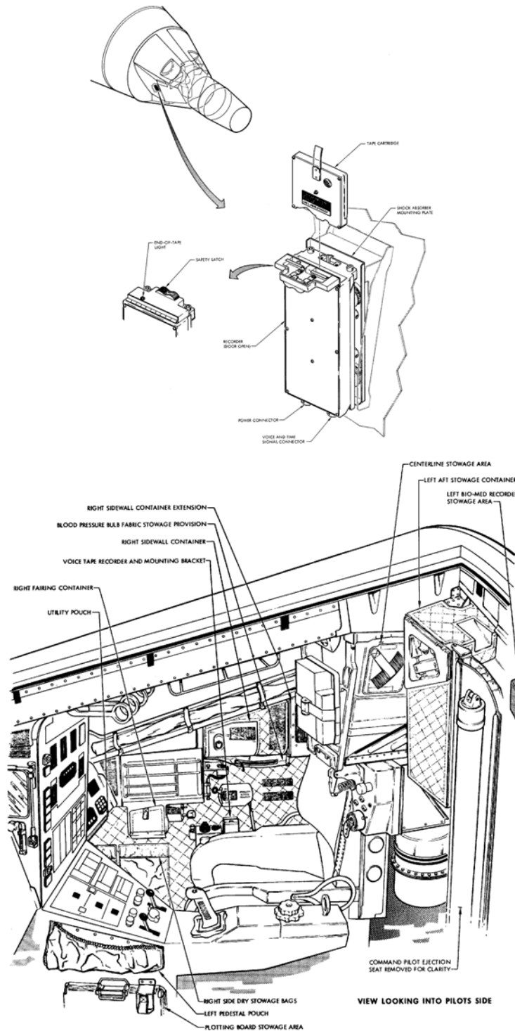
Figure 4 - These two drawings show the onboard Gemini voice tape recorder and the relative position of the unit inside the Gemini cockpit. The actual position of the tape recorder varied from spacecraft to spacecraft. Drawings taken from the "NASA Project Gemini Familiarization Manual, Long Range and Modified Configurations," Manned Satellite Spacecraft, McDonnell, SEDR 300 Volume 1, September 30, 1965.
