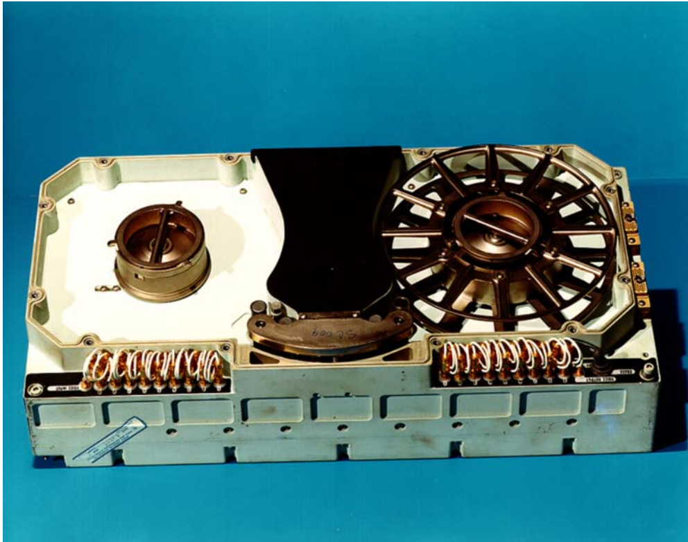
Figure 5 - The Apollo Command Module's onboard Data Storage Equipment (DSE) is shown here with outer cover removed. Shown at right is one of two eight-inch reels that spooled the 2,250-feet of one-inch Mylar magnetic tape through the 14-track read-write heads. The DSE was a self contained unit housed in the CM's lower equipment bay. NASA Photo No. S66-22993.
