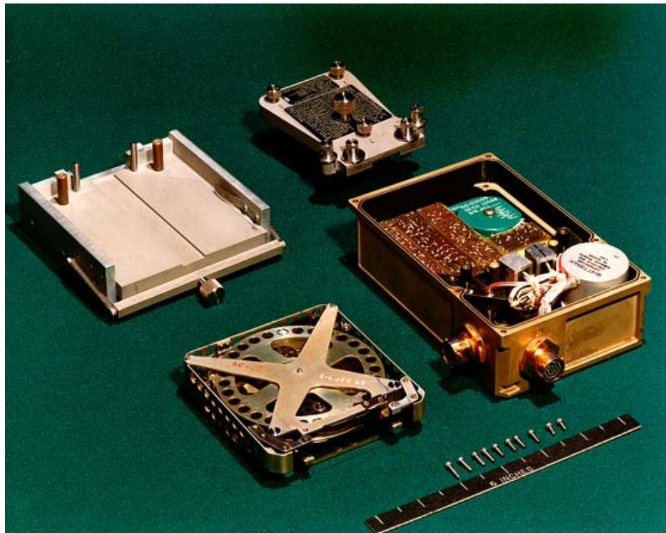
Figure 7 - The Lunar Module's onboard Data Storage Electronics Assembly (DSEA). Top photo shows the finished unit. Bottom photo shows the DSEA, with cover and tape cartridge removed, revealing the interior electronics. Note the tape cartridge loader tool in the upper right portion of the bottom photo. NASA Photo No. S73-37044 and S73-37047.
